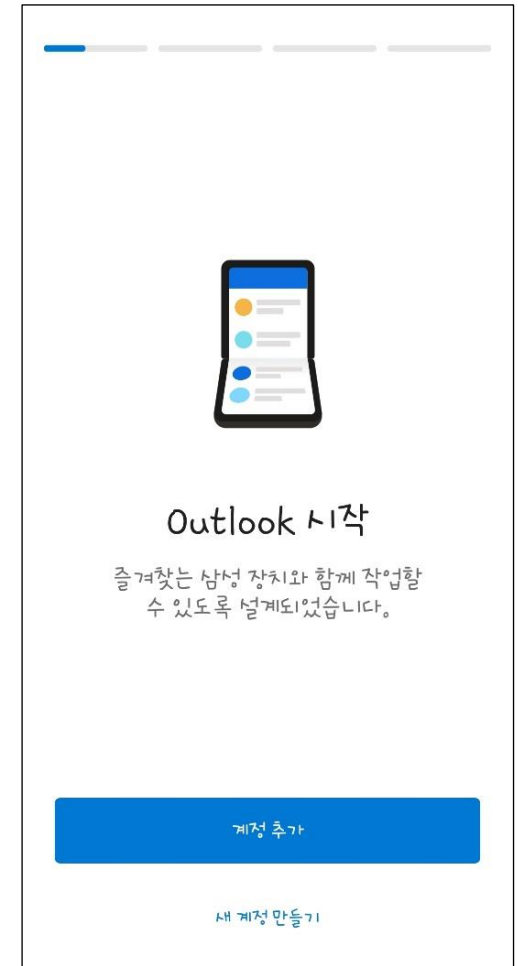
Outlook
